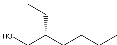
FIG. 1 - Structure of (R)-(-)-2-ethylhexan-1-ol.
